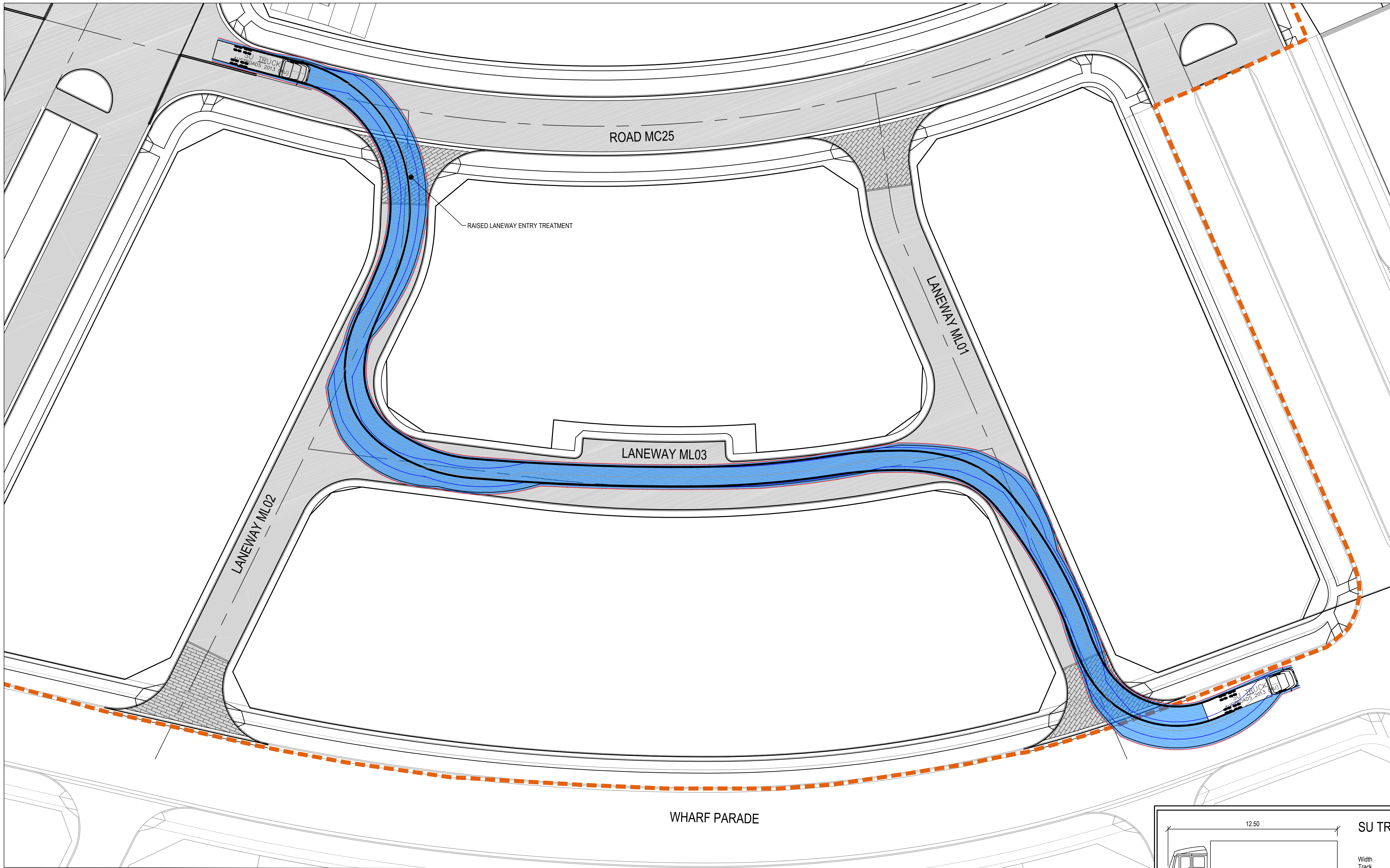
ROAD ML02 - ML03- ML01 GARBAGE TRUCK SWEEP PATH SCALE 1 : 250
